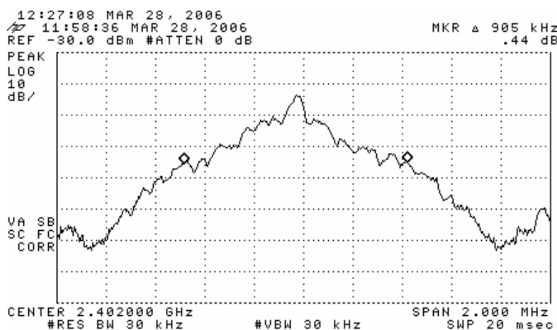
Figure 6.1 Measurement of channel 20 dB bandwidth. (top) Low Channel, (middle) Middle Channel, (bottom) High Channel
